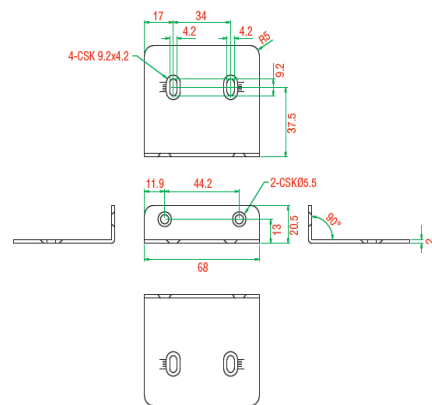
Port P06HC's L-type mounting kit
